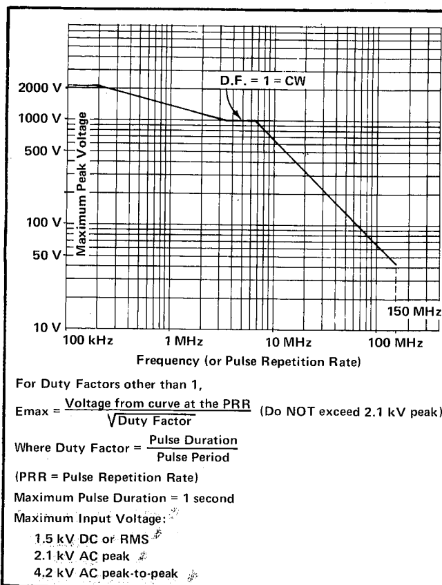
Fig. 3. P6009 Probe, maximum input voltage versus frequency.
