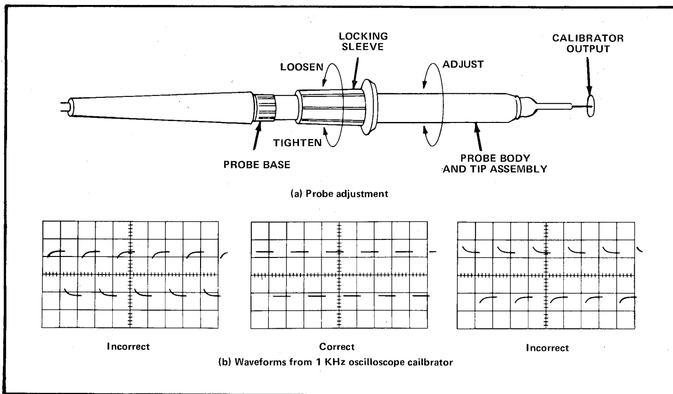
Fig. 5. Probe L.F. Compensation.
